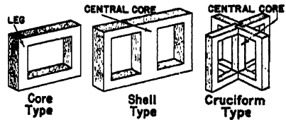
Core constructions for transformers.
